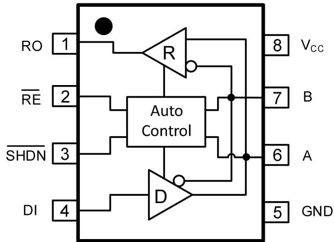
Figure 1 Pin Diagram
