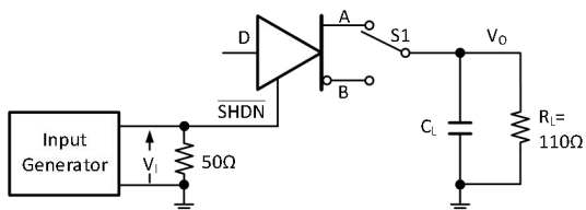
Figure 4. Measurement of Driver Enable and Disable Times with Active High Output and Pull-Down Load
