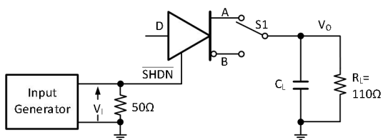
Figure 4. Measurement of Driver Enable and Disable Times with Active High Output and Pull-Down Load
