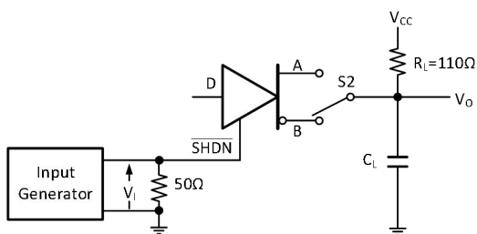
Figure 5. Measurement of Driver Enable and Disable Times with Active Low Output and Pull-up Load
