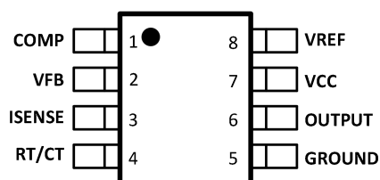
Pin Diagram
